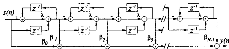
Fig. 11. WFIR filter where unit delays of a conventional filter are replaced with first-order all-pass filters D(z) . Term WFIR illustrates structural similarity with a nonwarped FIR filter.
