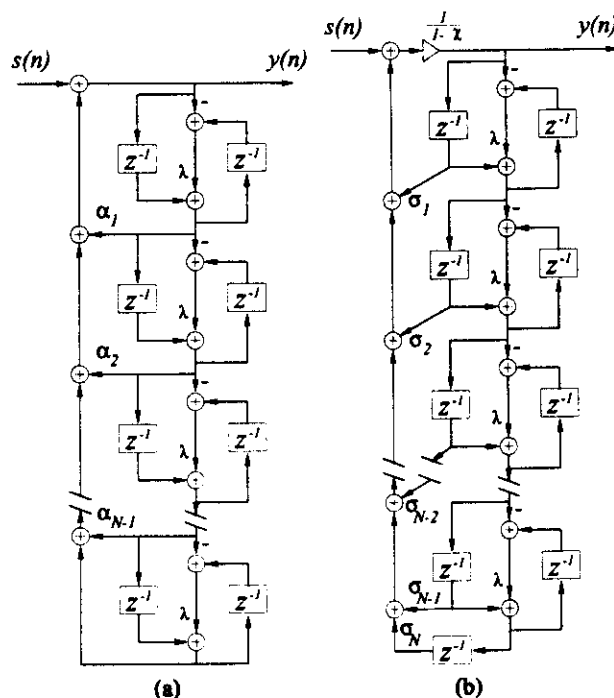
Fig. 13. (a) WIIR filter, which cannot be implemented directly because it has delay-free recursive loops. (b) Directly realizable WIIR filter.
