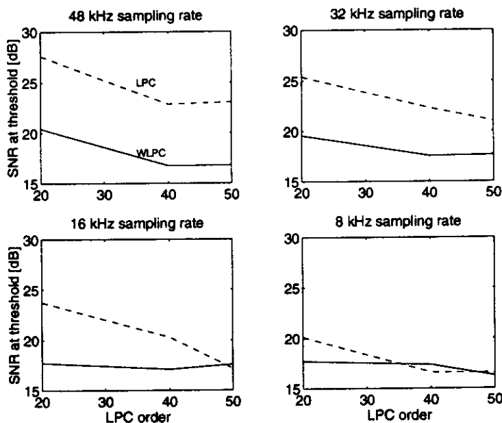
Fig. 21. Preliminary listening test results at four different sampling rates as a function of the order of a WLPC and an LPC filter. Only average data over 11 test signals and two subjects are shown.
