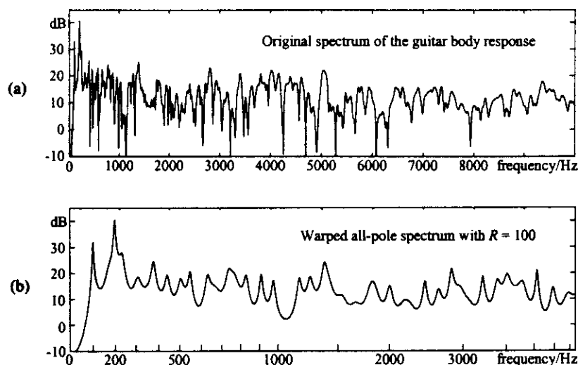
Fig. 23. Modeling of guitar body response. (a) Original magnitude response. (b) Magnitude response using WIIR modeling (notice warped frequency scale).
