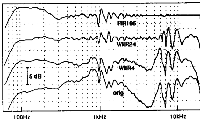
Fig. 22. Loudspeaker equalization curves. orig—original magnitude response; WIIR4, WIIR24—WIIR equalization, filter orders 4 and 24; FIR105—FIR filter equalization, filter order 105.
