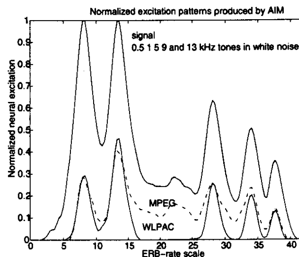
Fig. 20. Noise processes in WLP coding. The original signal consists of a set of sinusoids and white background noise. The error has the same spectral shape as the original signal due to open-loop coding scheme. The corresponding coding error signal in an MPEG I layer 3 codec is plotted for comparison (---).
