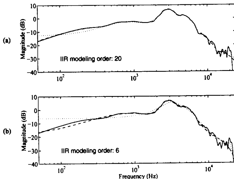
Fig. 24. Example of modeling minimum-phase dummy-head HRTFs using warped IIR filters: (a) filter order 20. (b) order 6. (—) original HRTF magnitude response. (····) IIR model using Prony's method. (---) warped IIR model using Prony's method (warping coefficient 0.65). Warped IIR models have been unwrapped to second-order sections to retain the same computational complexity as linear designs.
