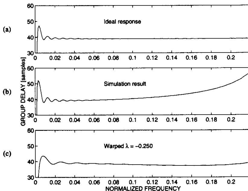
Fig. 26. Group delays corresponding to impulse responses in Fig. 25.
