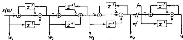
Fig. 6. Direct-form II implementation of all-pass chain.
