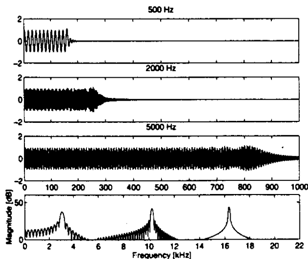
Fig. 8. Set of warped signals and their sum spectrum.
