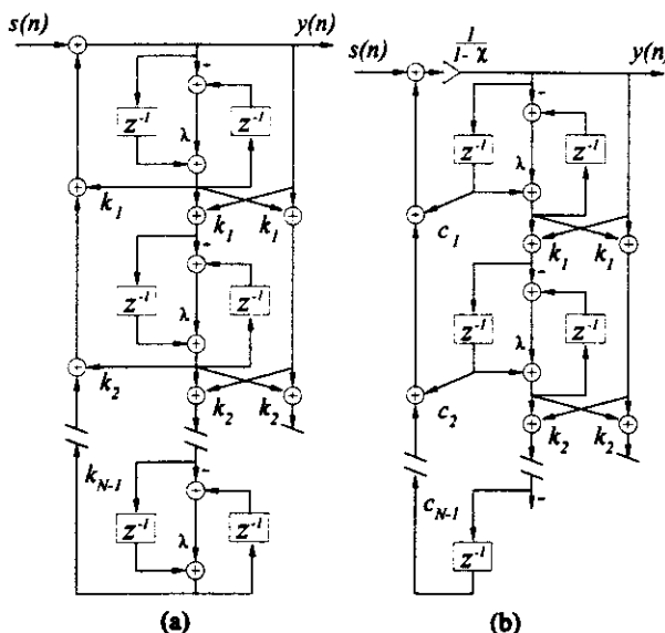
Fig. 14. (a) WIIR lattice filter, which cannot be implemented directly because it contains delay-free recursive loops. (b) Directly realizable WIIR lattice filter.
