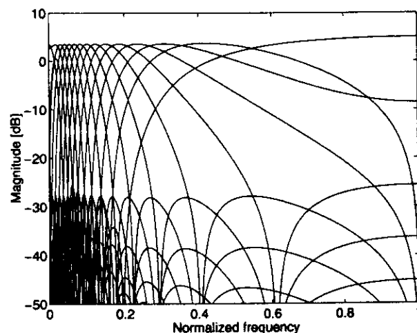
Fig. 16. Example of frequency responses of 16-channel warped filter bank. Filter bank was designed using an all-pass filter chain of 16 elements, and Hamming windowing was used prior to FFT.
