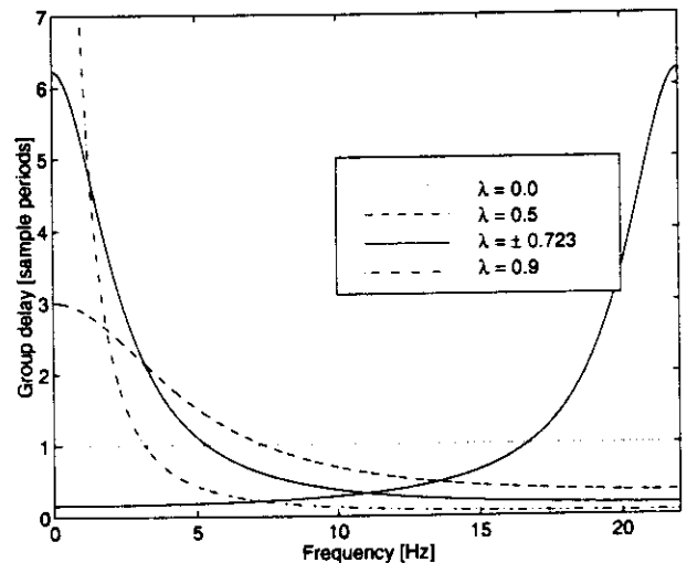
Fig. 5. Group delay of first-order all-pass filter.
