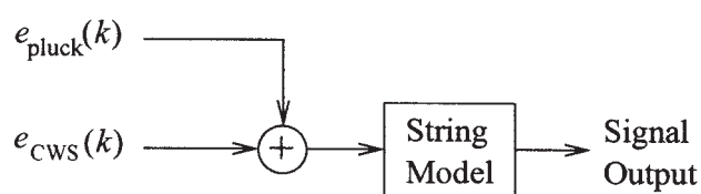
Fig. 2. Bandwidth extension scheme.
