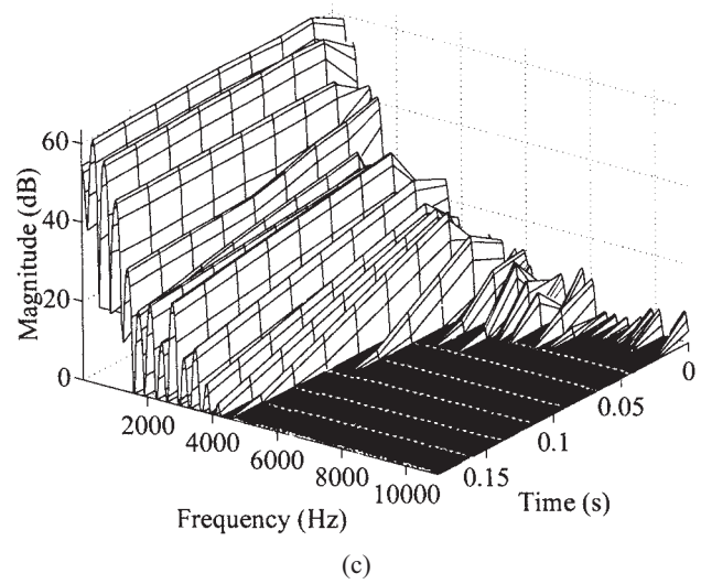
Fig. 6. Time–frequency analysis. (a) Original tone. (b) Low-pass-filtered tone. (c) Resynthesized tone.
