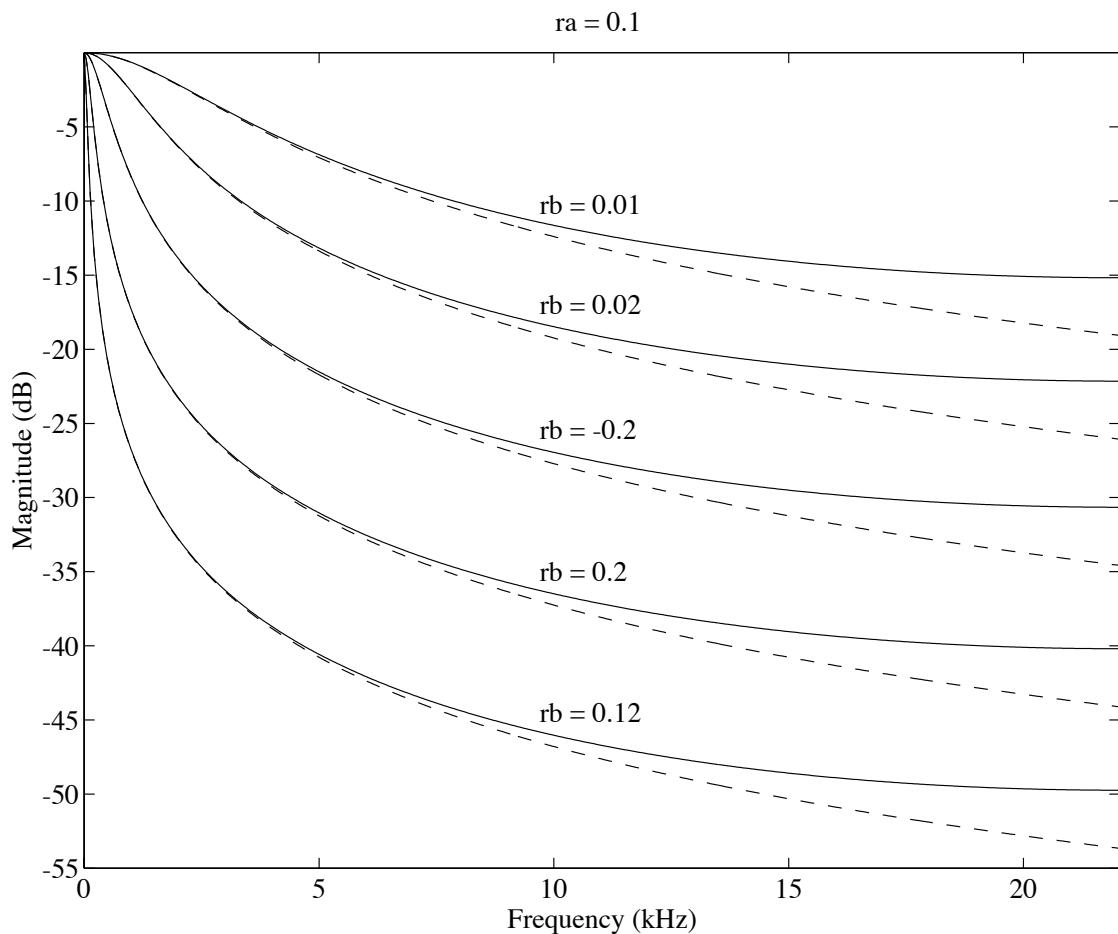
Fig. 2.16 Magnitude responses of the analog (dashed lines) and digital (solid lines) reflection functions with taper discontinuity only. The sampling rate is 44.1 kHz.
